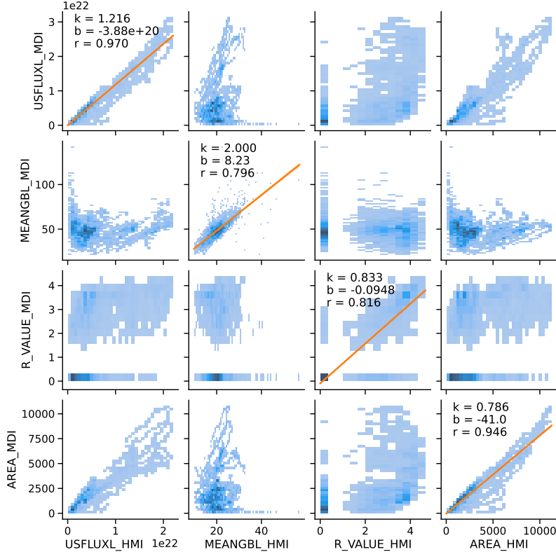
Figure 2. 2D histograms of summary parameters USFLUXL , MEANGBL , R.VALUE , and AREA between SHARP and SMARP. SHARP summary parameters are suffixed with _HMI and SMARP with _MDI . The orange lines in the diagonal blocks are the least square fit of SMARP summary parameters on the corresponding SHARP summary parameters, with coefficient k , intercept b , and Pearson correlation coefficient r displayed in the corner.
