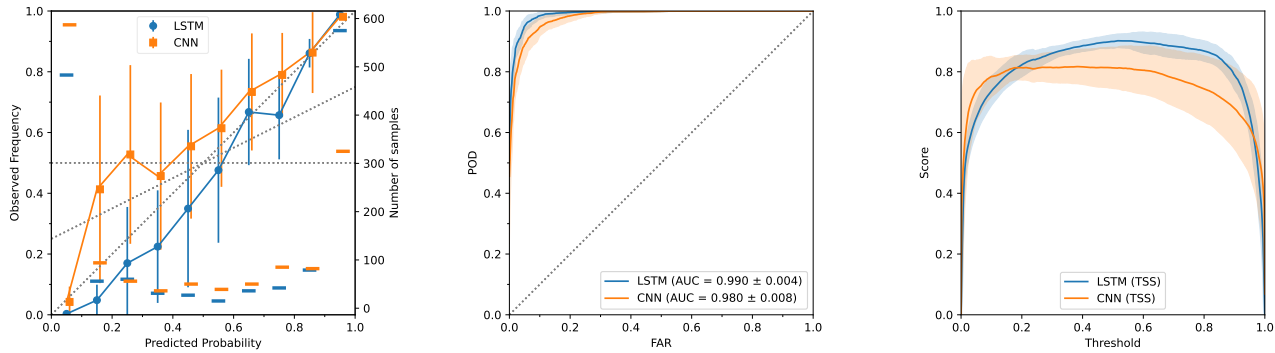
Figure 8. Verification plots of the LSTM and the CNN on FUSED_SHARP. Shown are the reliability diagram, ROC, and SSP, from left to right. This figure essentially extracts the blue curves (representing FUSED_SHARP) in both rows of Figure 6 and overlaps them together.
