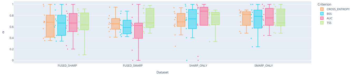
Figure 10. Stacking weight \alpha fitted using different criteria on different datasets. All 10 values of \alpha in an experiment setting are shown as points next to the corresponding box.
